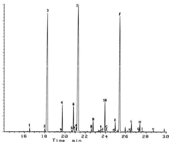
Fig. 5. Example of a gas chromatogram of a single Dufour gland of P. species A worker on the HP-1 coated column. For identification of peaks, see Table.
